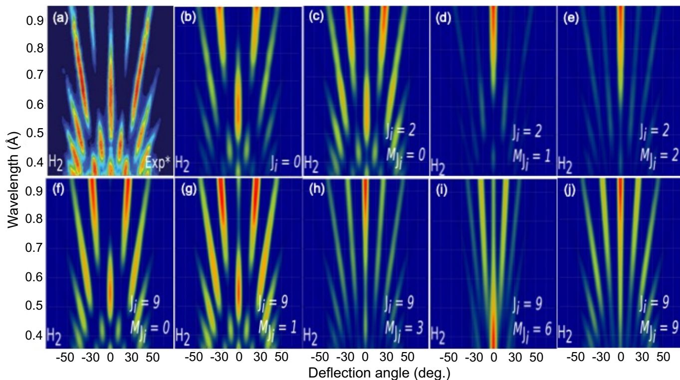
Fig. 6 \text{H}_2/\text{KCl}(001) GIFMD patterns along the crystallographic direction [100] . (a) Experimental pattern (data taken from ref. 67 ); (b), (c), (d), (e), (f), (g), (h), (i) and (j) simulated pattern for (J = 0, M_J = 0) , (J = 2, M_J = 0) , (J = 2, M_J = 1) , (J = 2, M_J = 2) , (J = 9, M_J = 0) , (J = 9, M_J = 1) , (J = 9, M_J = 3) , (J = 9, M_J = 6) and (J = 9, M_J = 9) , respectively.
