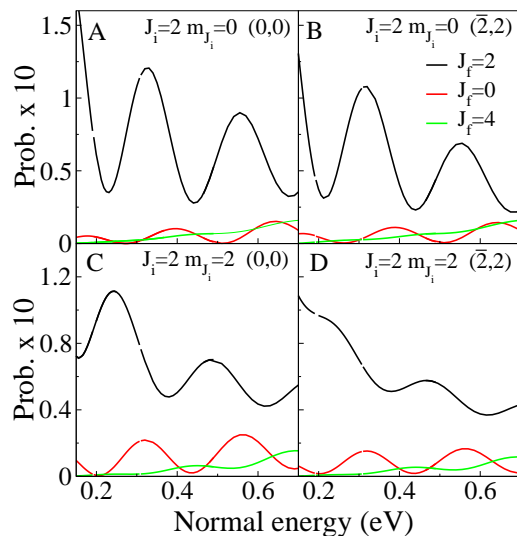
Fig. 8 Elastic (black line) and rotationally excited and deexcited probabilities (green and red lines) as a function of the normal incidence energy. The diffraction peak and the initial rotational state is shown in the legends. In all four case, the molecules are in the vibrational ground state.
