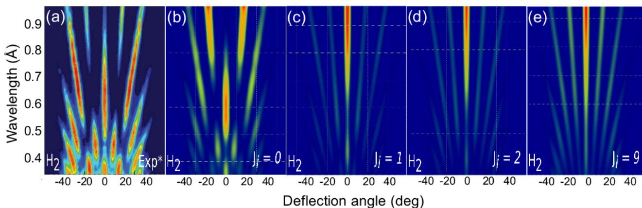
Fig. 5 \text{H}_2/\text{KCl}(001) GIFMD patterns along the crystallographic direction [100] . (a) experimental pattern (data taken from ref. 67 ); (b), (c), (d), and (e) simulated pattern for J = 0 , J = 1 , J = 2 , and J = 9 , respectively.
