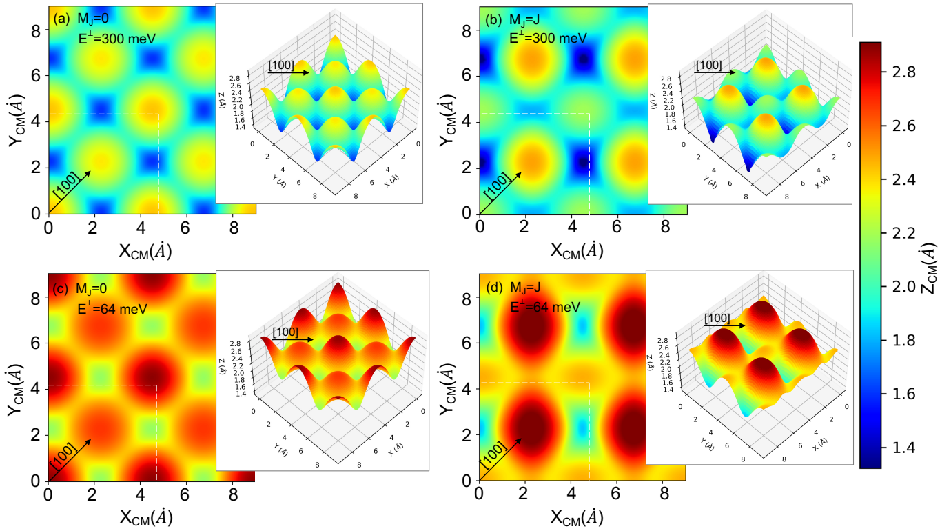
Fig. 7 2D and 3D (insets) representations of the classical turning points ( Z(\text{\AA}) ) for cartwheel ( M_J=0 ) and helicopter ( M_J=J ) molecules for two perpendicular kinetic energies ( E^\perp ). The squares delimited by white dashed lines represent the KCl(001) unit cell -see Fig. 1. Note that E^\perp = 64 and 300 meV correspond to \lambda^\perp = 0.8 and 0.37 Å, respectively.
